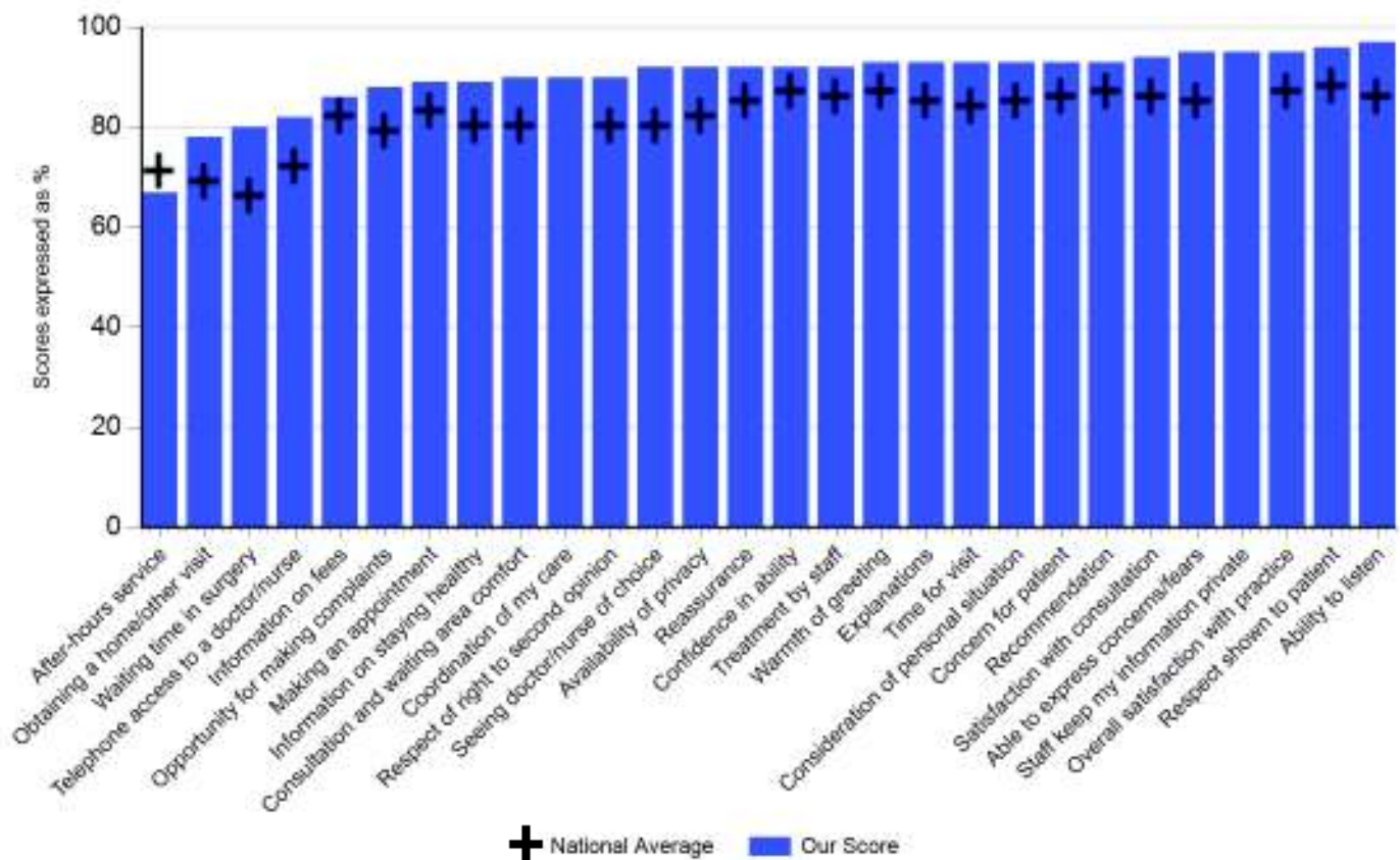
Overall scores
